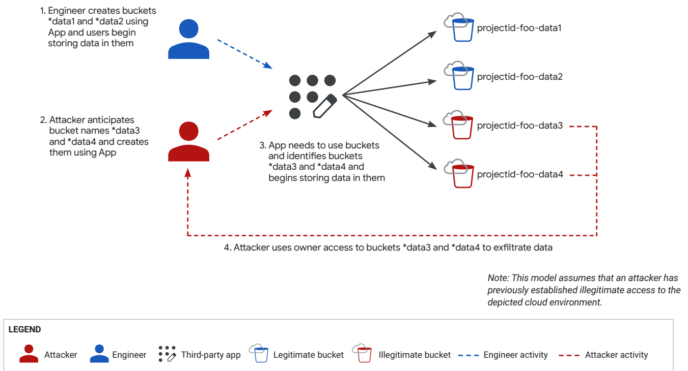
Figure 2: Model of a Cloud Storage Bucket Naming Convention Exploited by a Threat Actor
