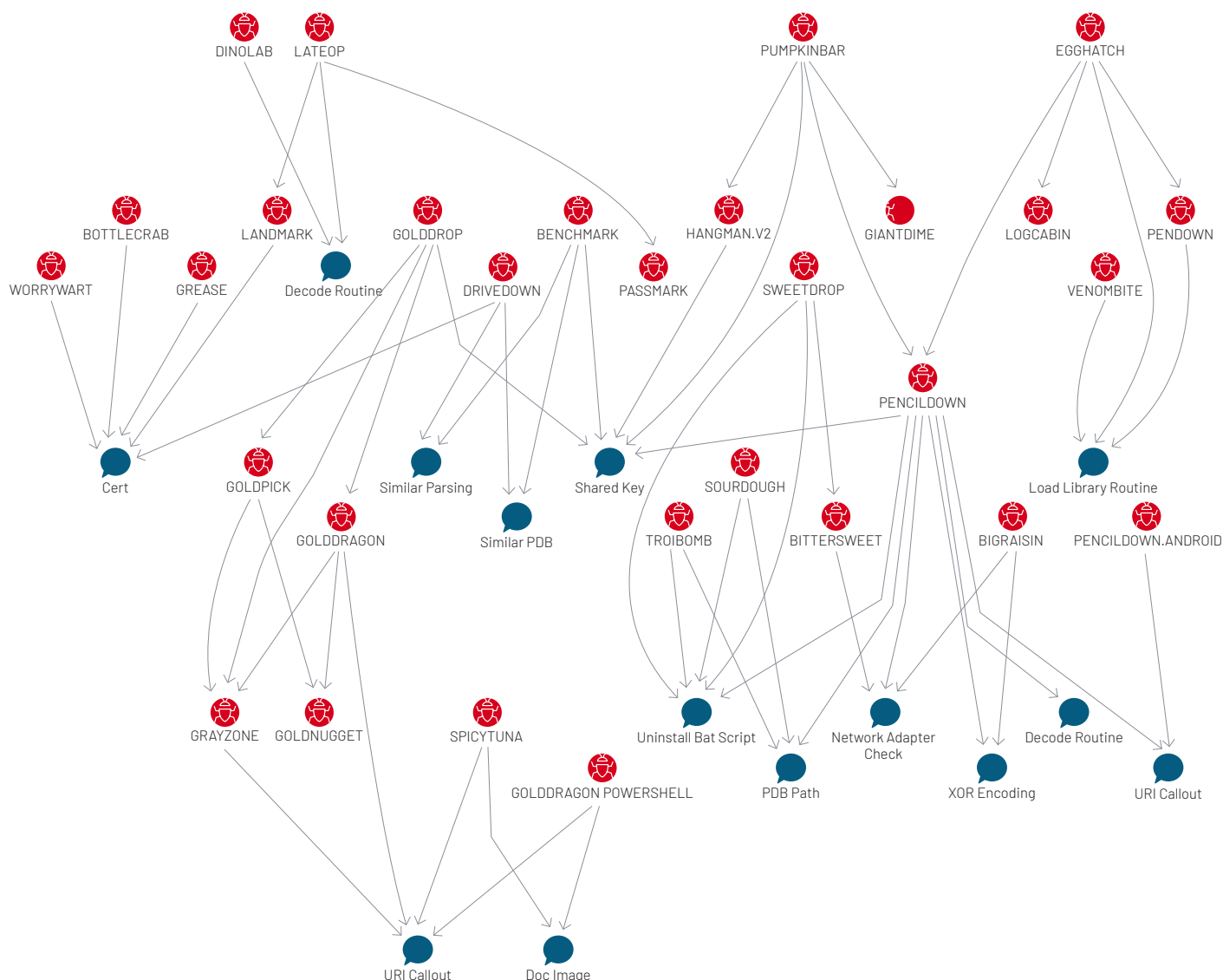
FIGURE 8. Code family overlap across tools used by APT43.
